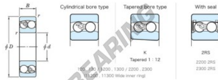
Spherical Ball Bearings-Open type-Open type AII
