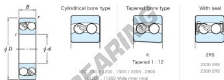
Spherical Ball Bearings-Cover type-Open type All
