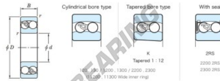
Spherical Ball Bearings-Cone type-Open type All
