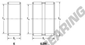
Basic roller and cage assemblies
