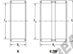
Radial inside roller and cage assemblies
