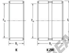
Back needle roller and cage assemblies
