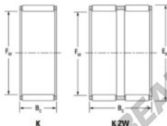
Bead of needle roller and cage assemblies
