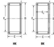
Main series with cage assembly
