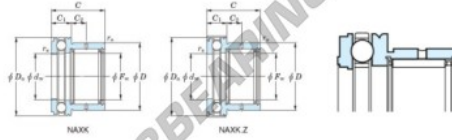
Boundary dimensions
