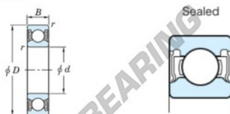
Contact sealed
