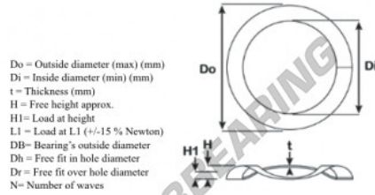
Overlap Wave Spring Washers
