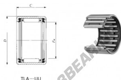
Shell Type needle roller with seals
